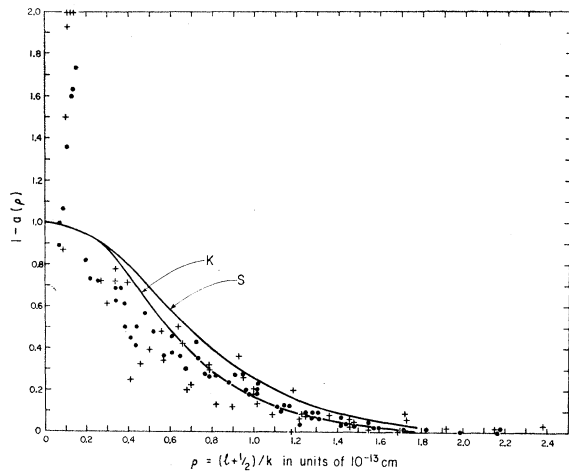
FIG. 8. Plot of 1-a_l(\rho) versus \rho where \rho = (l+\frac{1}{2})/k . \rho is in units of 10^{-13} cm and k is the wave number in the barycentric system. Plus signs are for all the \pi^+ + p data analyzed in this paper except the 1.33 GeV/c \pi^+ + p , and filled circles are for all the \pi^- + p data. S designates the curve for 19.6-GeV/c p + p elastic scattering derived from the analysis of Serber in Ref. 20. K designates the curve given by Krisch in Ref. 19 for p + p elastic scattering above 10 GeV/c.
